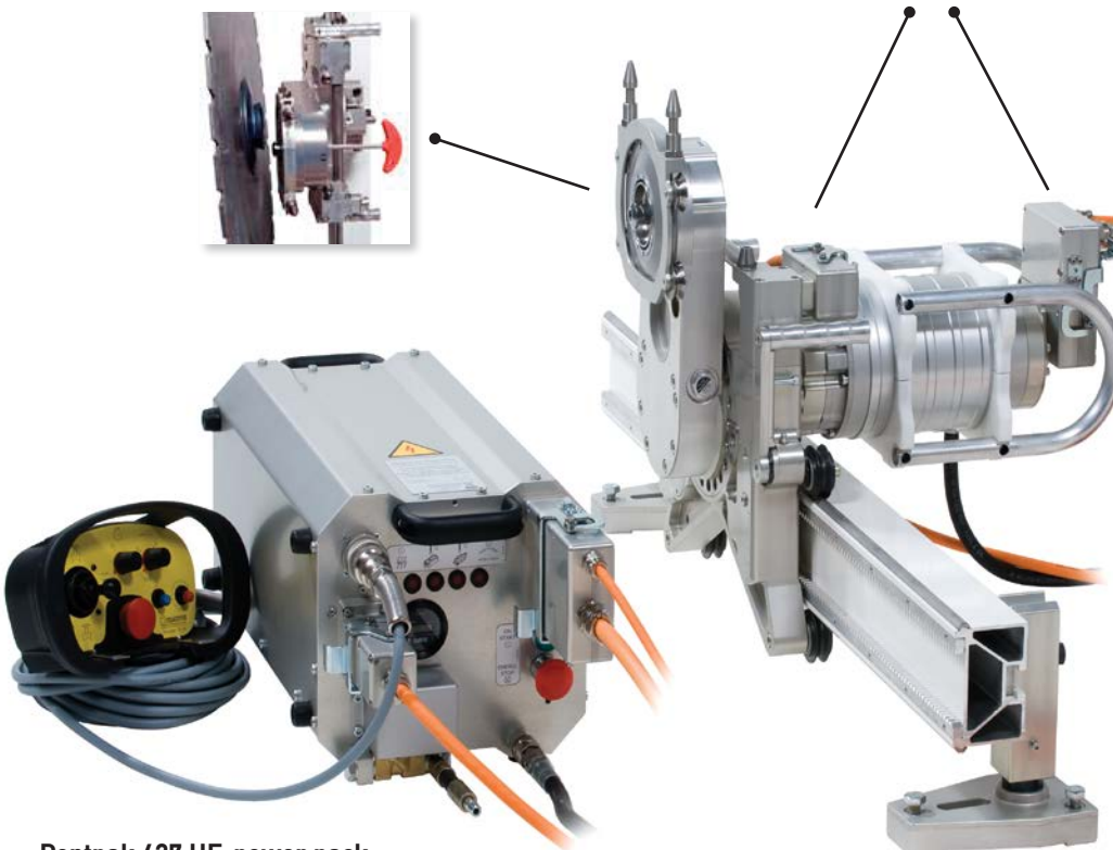
Pentpak 427 HF-power pack with Pentruder autofeed system
